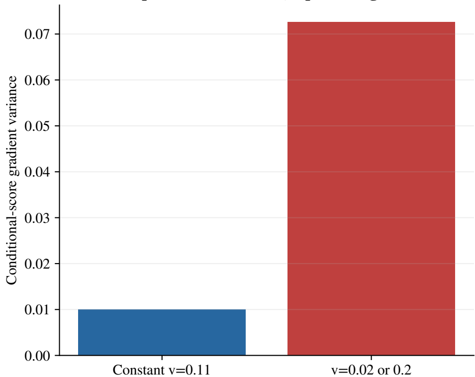
Equal mean variance, equal marginal
