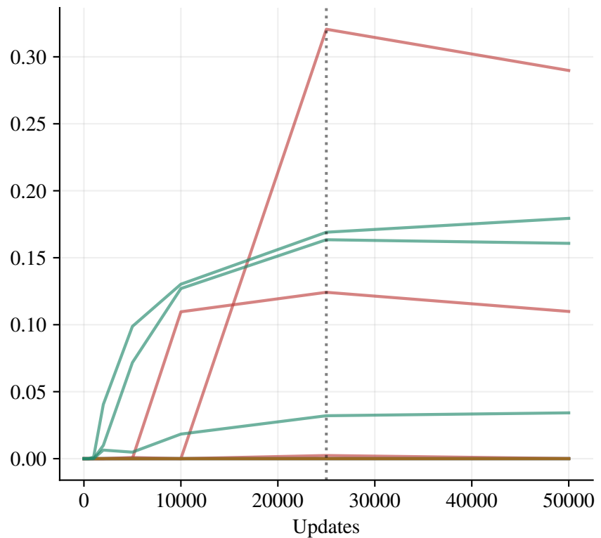
Fraction at canonical floor (0.0001)
