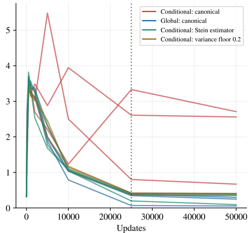
Sliced Wasserstein distance
