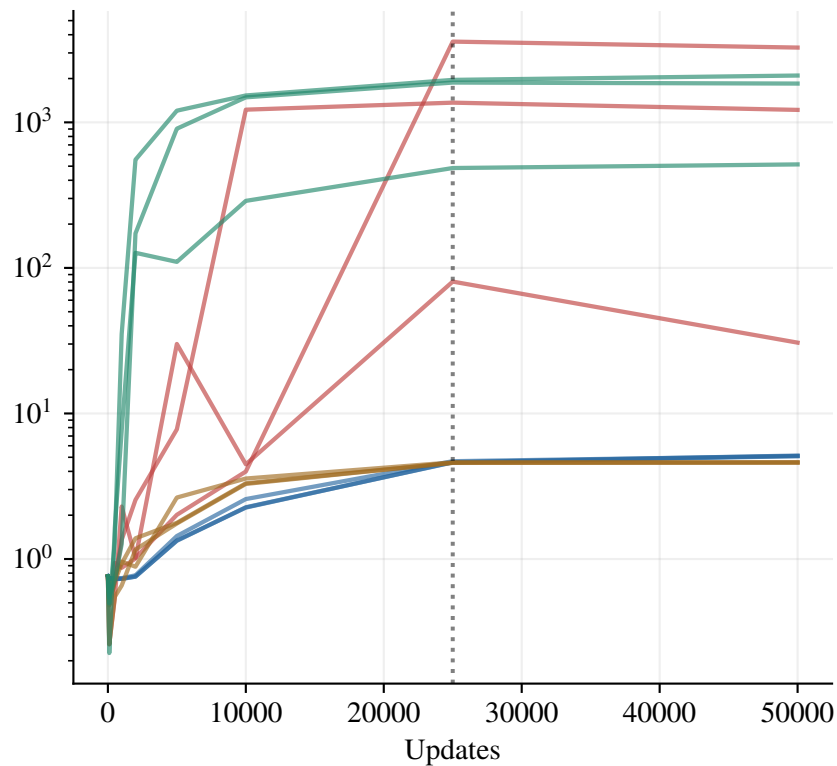
Mean inverse conditional variance
