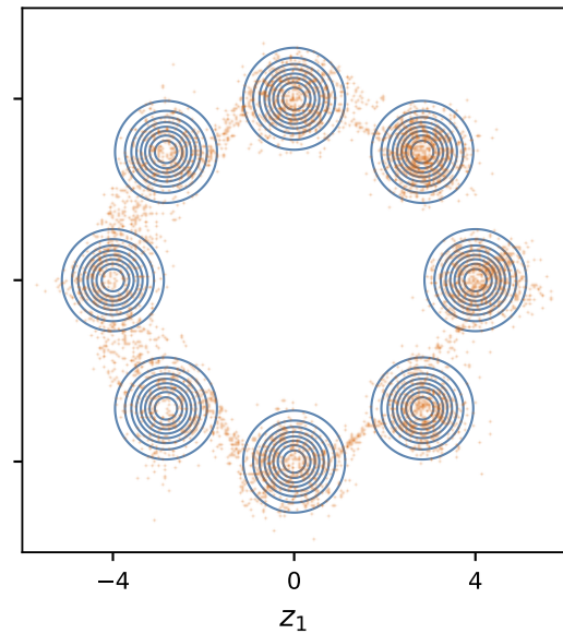
RealNVP-16 seed 46 · ELBO -0.291 · SW 2 0.393
