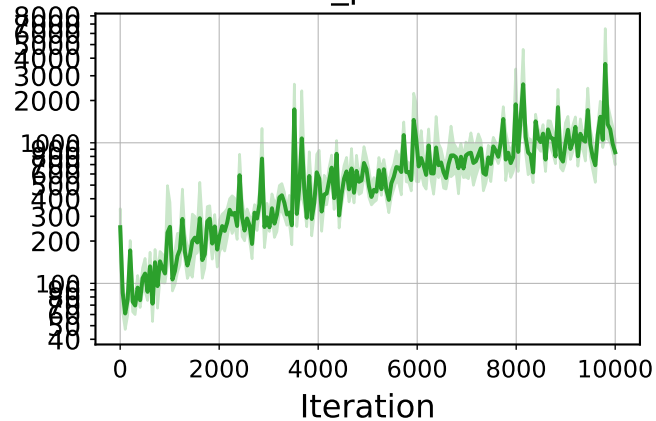
Bnn_protein
