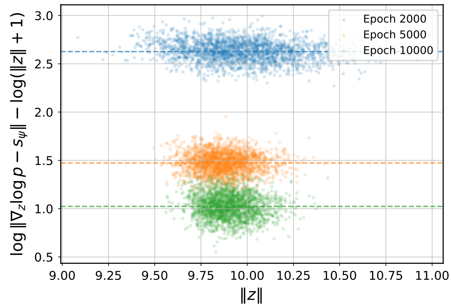
Conditioned Diffusion
