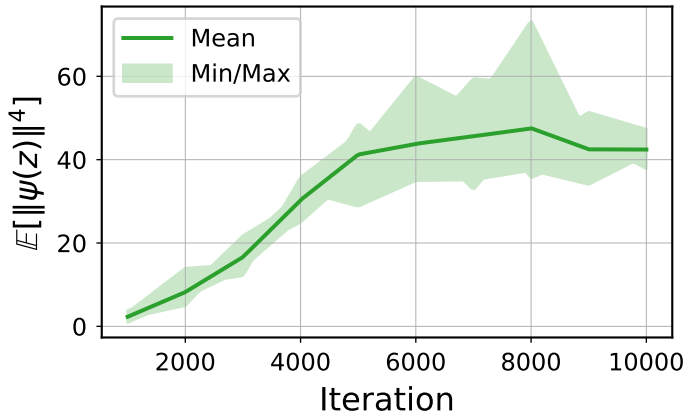
x_shaped
