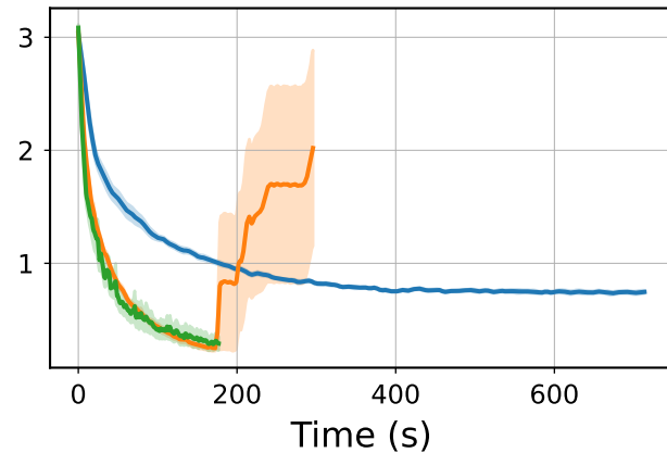
8_gaussians
