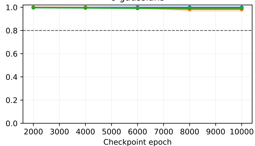
8 gaussians
