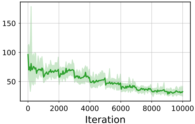
Conditioned Diffusion
