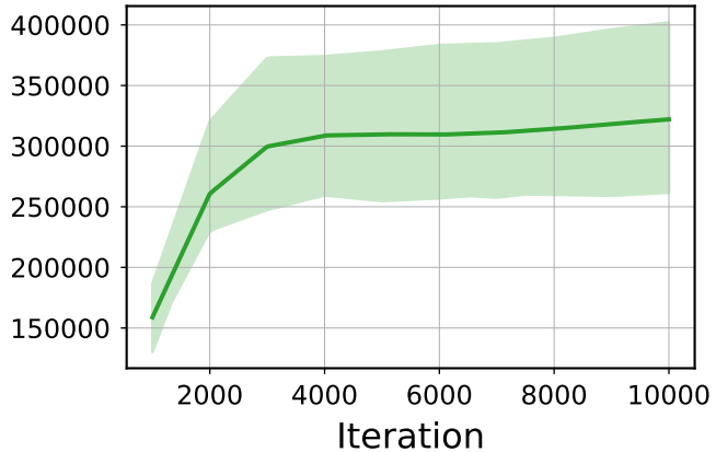
Conditioned Diffusion
