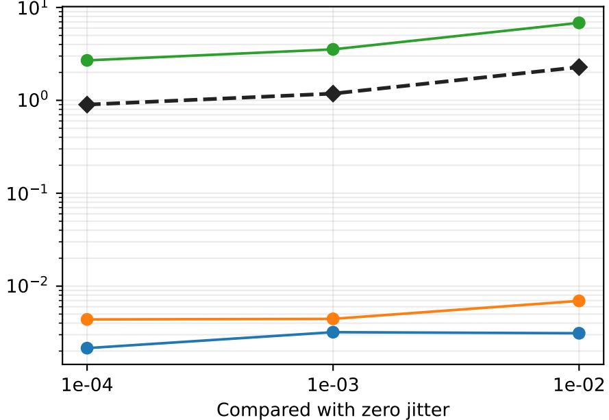
Pairwise HMC-reference L2
