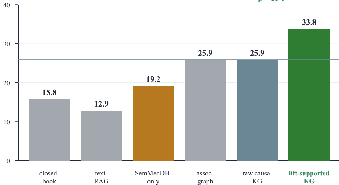
Causal-QA correctness (%)
