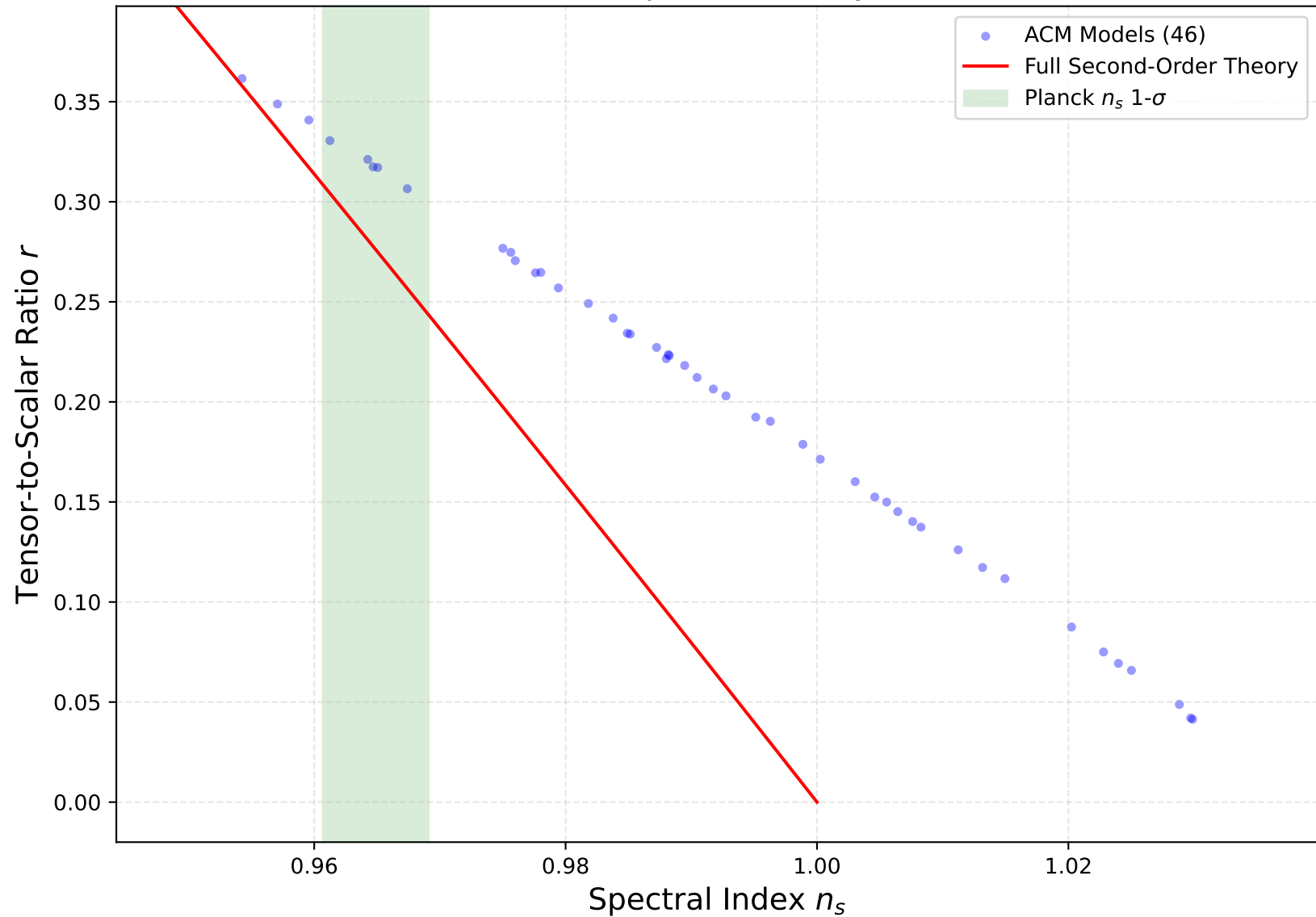
ACM Chaos Collapse vs. Analytic Attractor
