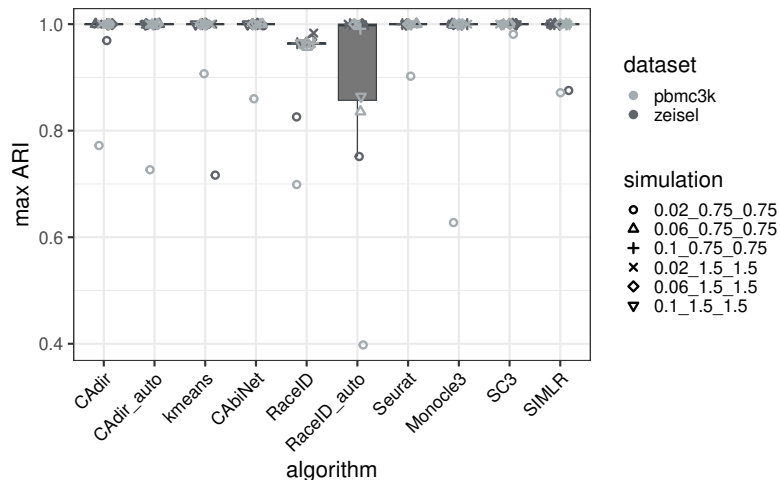
a Maximum ARI on simulated data
