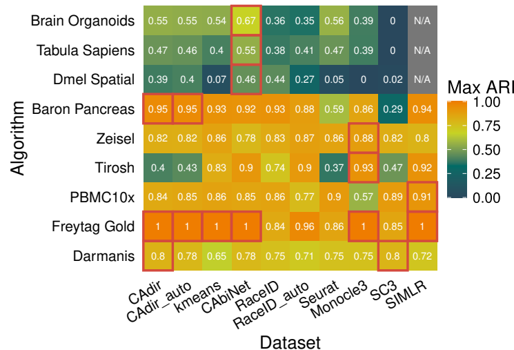
b Maximum ARI on experimental data
