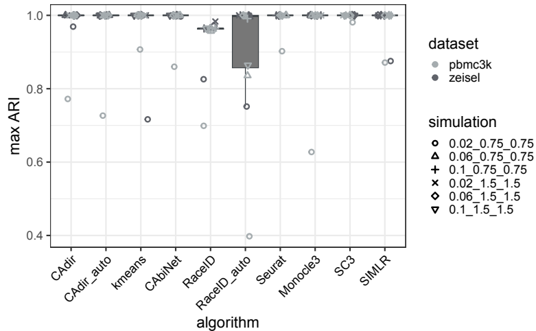
Maximum ARI on simulated data
