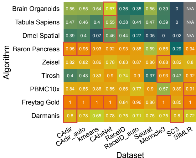
Maximum ARI on experimental data
