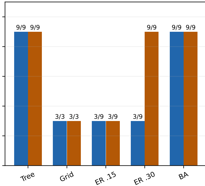
L(2,1)
