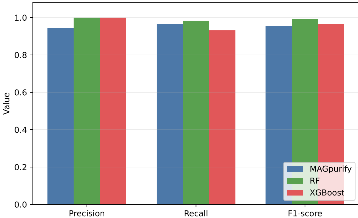
Sim-5G: MaxBin2 Correctness Metrics
