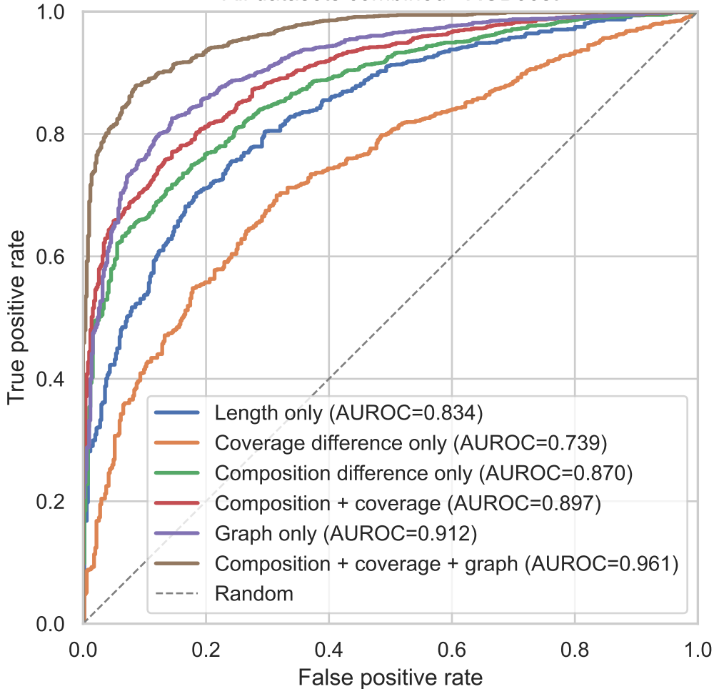
All datasets combined - XGBoost
