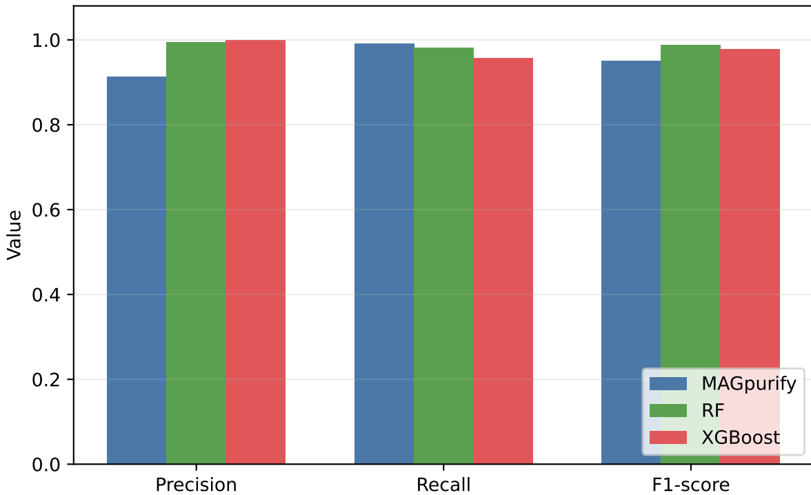
Sim-20G: MaxBin2 Correctness Metrics
