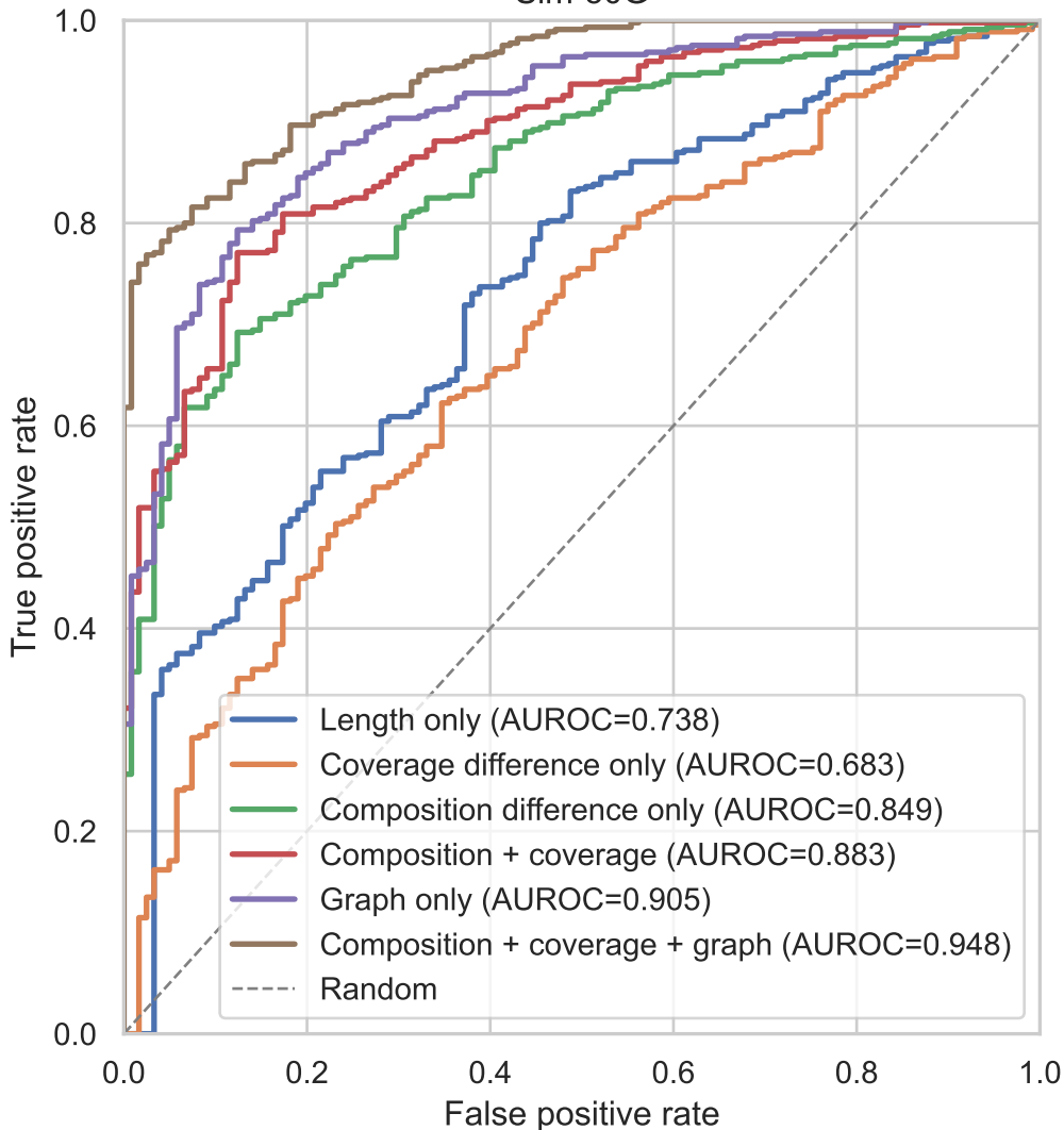
Sim-50G
