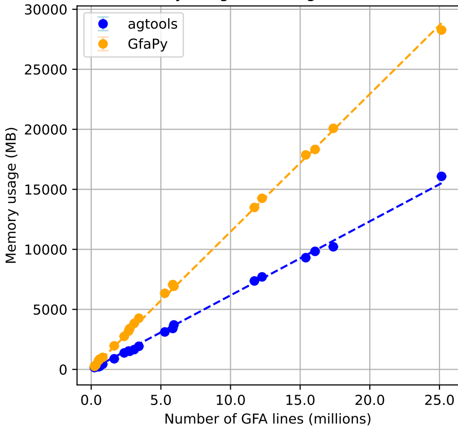
Memory usage - loading SPAdes GFA
