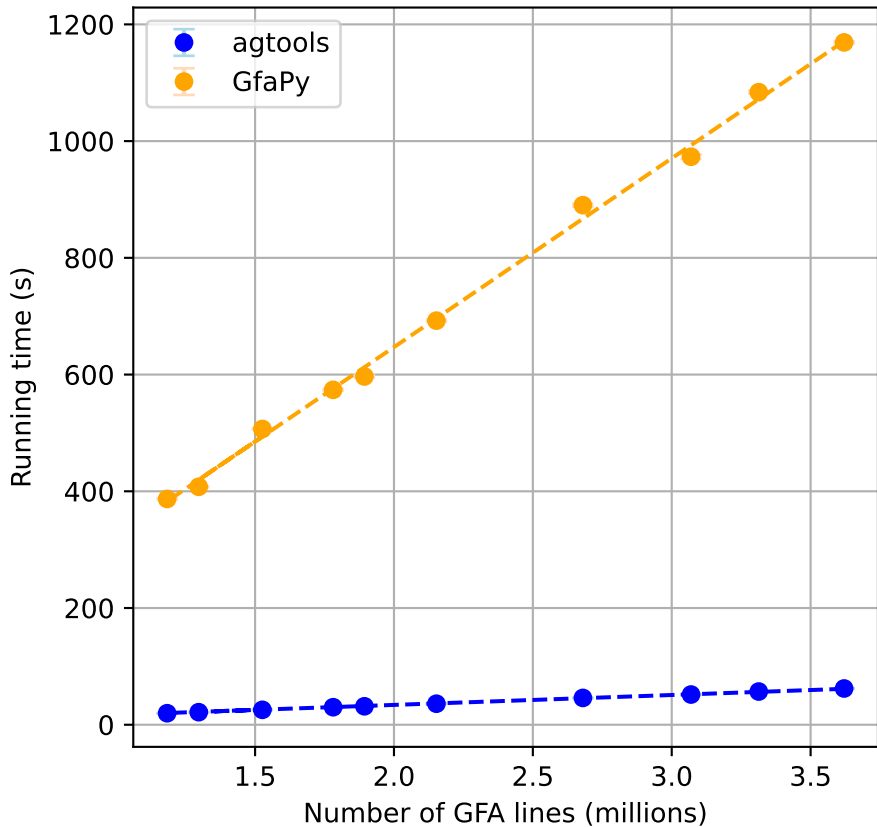
Running time - loading MEGAHIT converted GFA
