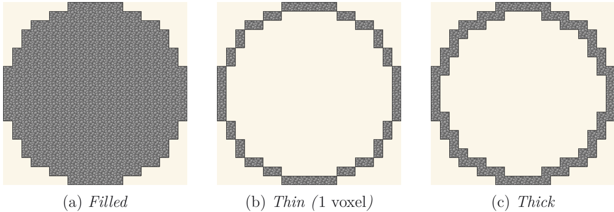
Figure 2: The three rendering modes for the same Euclidean circumference of D = 20 . The Thin mode corresponds to the discrete topological boundary ( \partial F ); the Thick mode adds diagonal cells to seal 45^\circ holes, essential for watertight builds (underwater Glass/Ice domes).
