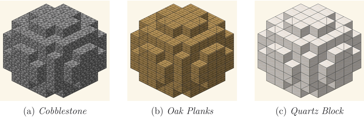
Figure 8: The same D = 8 sphere rendered with three different blocks. The voxelised silhouette (mathematics) is identical across all three: the algorithm picks the voxels; the texture is a purely aesthetic layer applied afterwards that changes neither volume nor topology.
