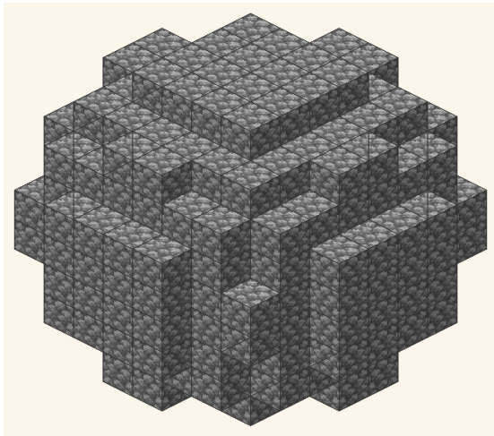
(a) Sphere D = 10, r_x = r_y = r_z = 5 .
