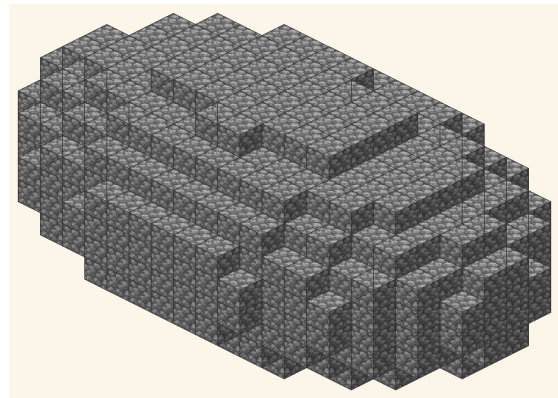
(b) Ellipsoid W = 20, H = 10, D = 12 .
