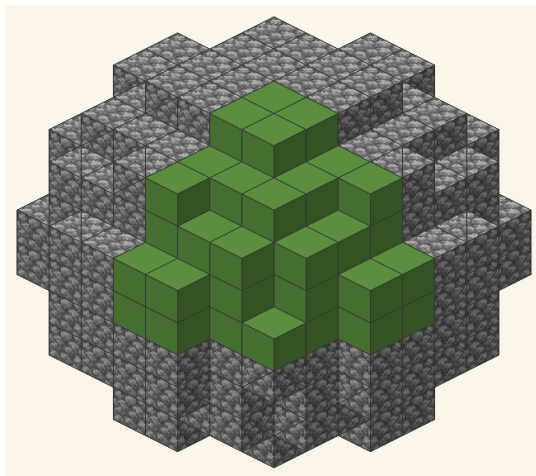
Figure 7: D = 10 sphere with positive octant (+x, +y, +z) highlighted in green. Under the action of the subgroup \mathbb{Z}_2^3 \leq O_h (order 8, generated by the three coordinate reflections), this octant determines the entire sphere — the other seven regions are obtained via a sequence of /clone calls with mode:masked applied to the manually built octant.
