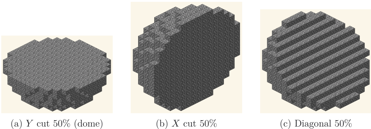
Figure 4: Three cuts on the same D = 16 sphere, each preserving 50% of the volume. The Y cut produces the classical dome V_{\text{dome}} = \frac{2}{3}\pi r^3 ; the diagonal exposes the hypotenuse x + y = k characteristic of that cutting plane.
