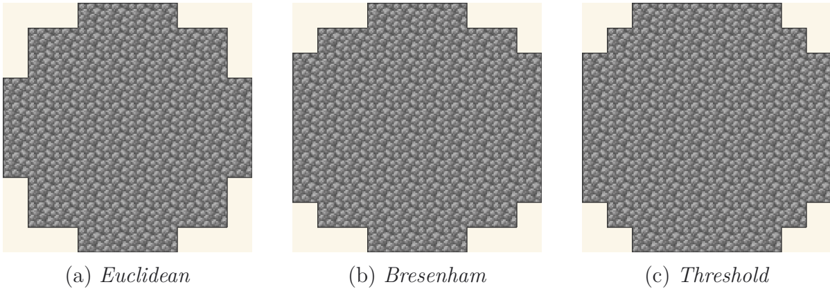
Figure 1: Same circumference of diameter D = 10 under the three criteria. Each figure shows the set of cells marked by the corresponding version of d_x^2 + d_y^2 \leq 1 , rendered with Minecraft cobblestone . Notice how the row transitions, corner cells and cardinal points differ — three mathematically correct answers under distinct criteria.
