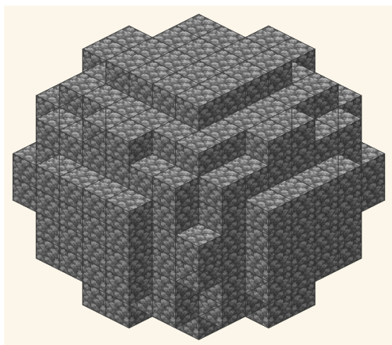
(a) Сфера D = 10, r_x = r_y = r_z = 5 .
