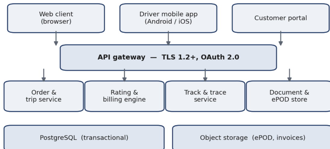
Figure 2.1: FleetLink application architecture. All client traffic passes through the API gateway; no client connects directly to a service or to the database.
