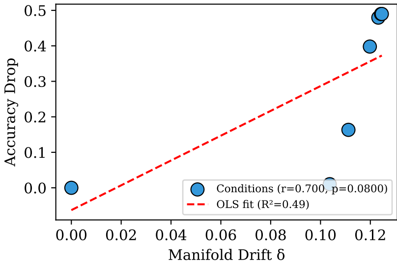
Figure 5 — Activation Drift vs Accuracy Drop (RQ2: \delta as Art. 9 risk predictor)
