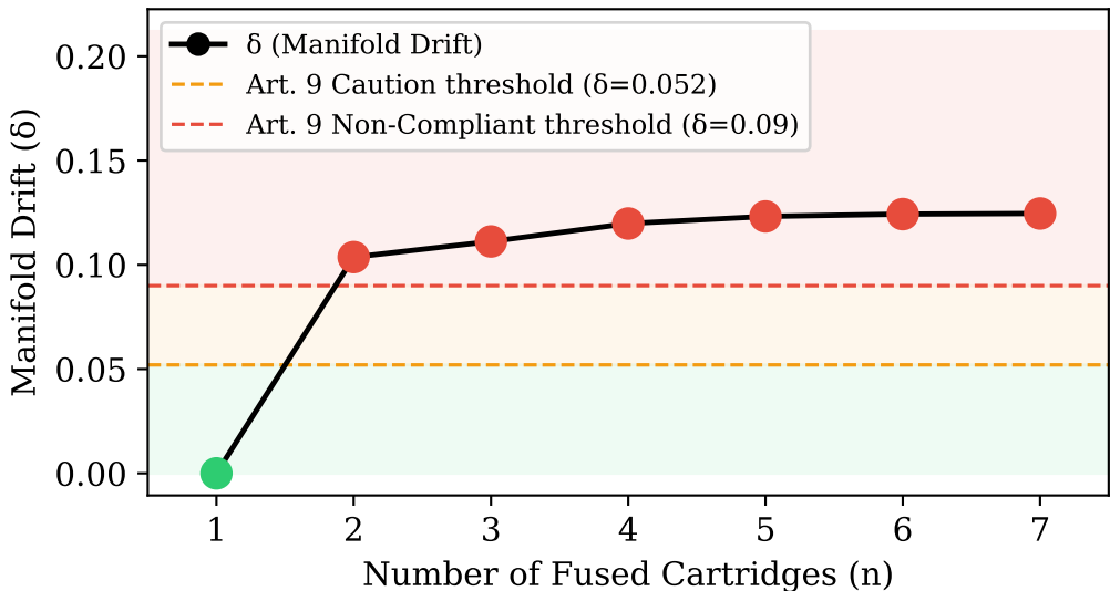
Figure 1 — Activation Space Drift vs Cartridge Count with EU AI Act Article 9 Risk Management Thresholds
