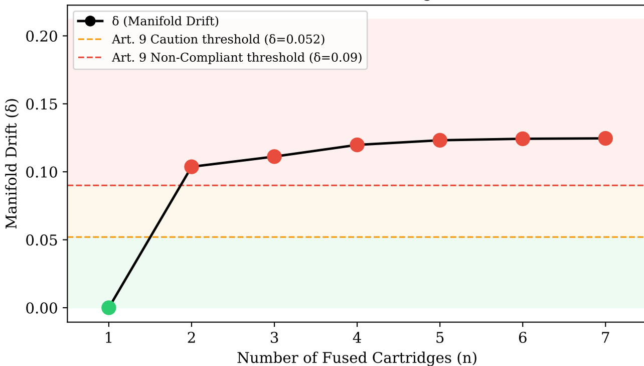
Figure 1 — Activation Space Drift vs Cartridge Count with EU AI Act Article 9 Risk Management Thresholds
