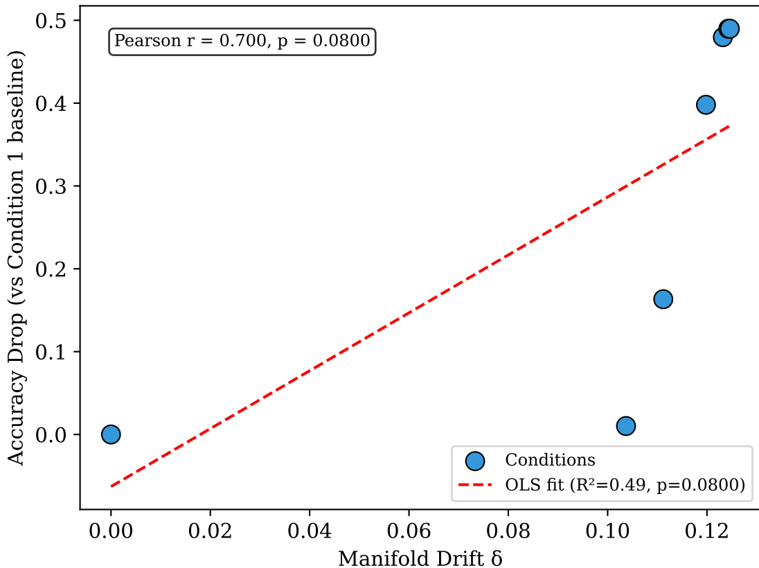
Figure 5 — Correlation: Activation Drift → Accuracy Degradation (RQ2: \delta as Art. 9 risk predictor)
