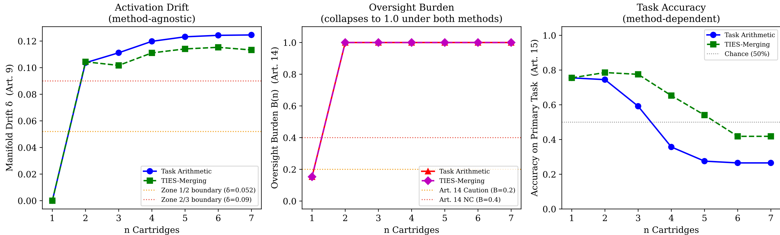
Figure 6 — Task Arithmetic vs TIES-Merging: \delta Detects Non-Compliance at n=2 While TIES-Merging Preserves Accuracy Beyond TA's Collapse Point
