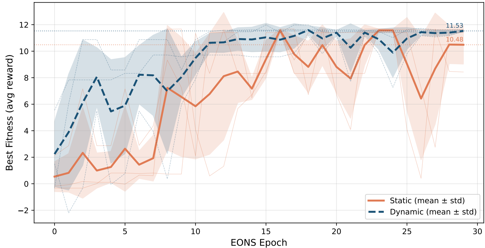
Hybrid SNN-EONS-DEAP: Learning Curves
