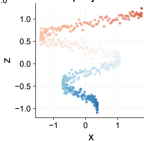
XZ projection
