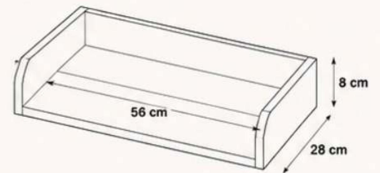
TOP TRAY DETAIL
