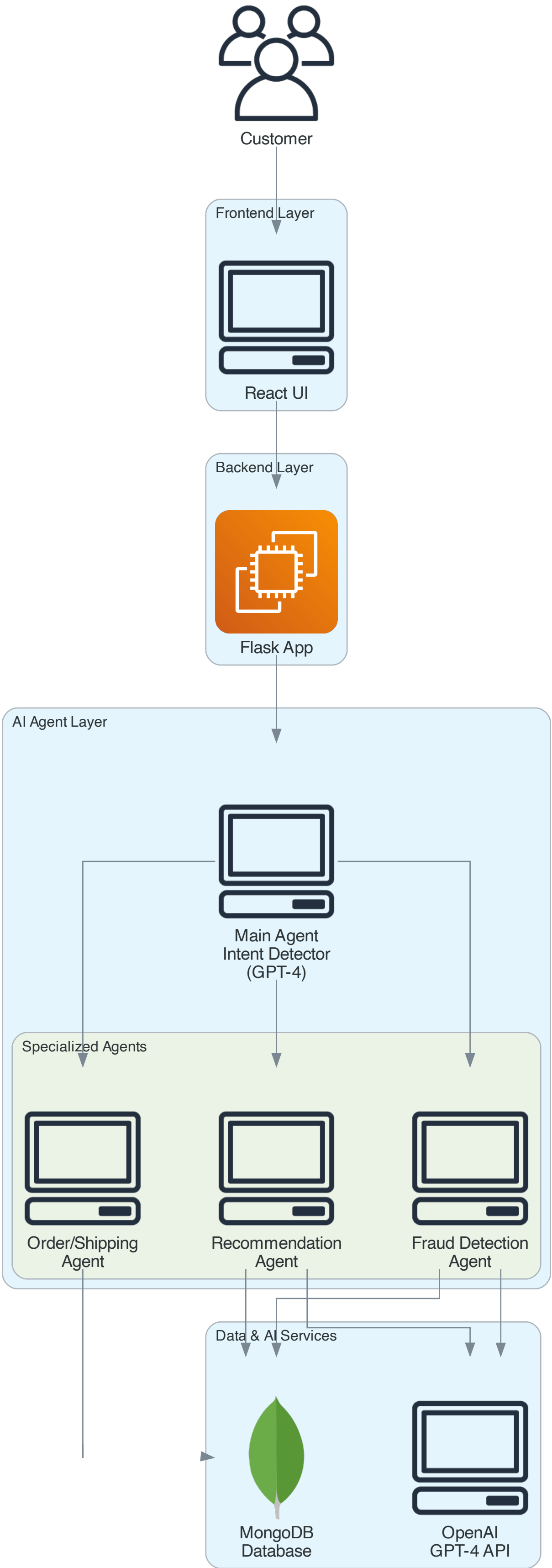
Multi-Agent AI System Architecture
