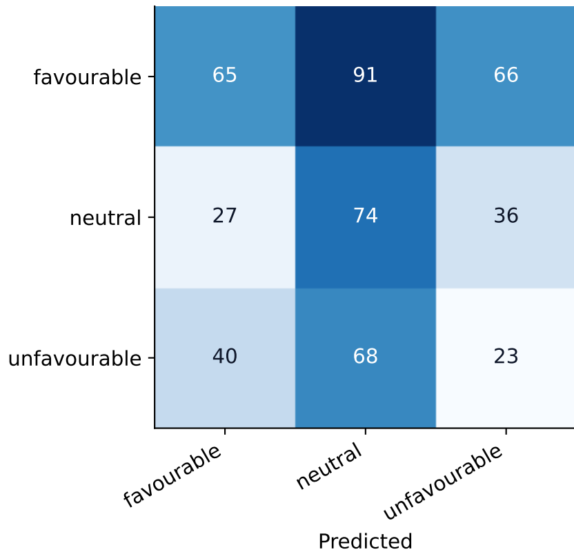
Pooled price random forest
