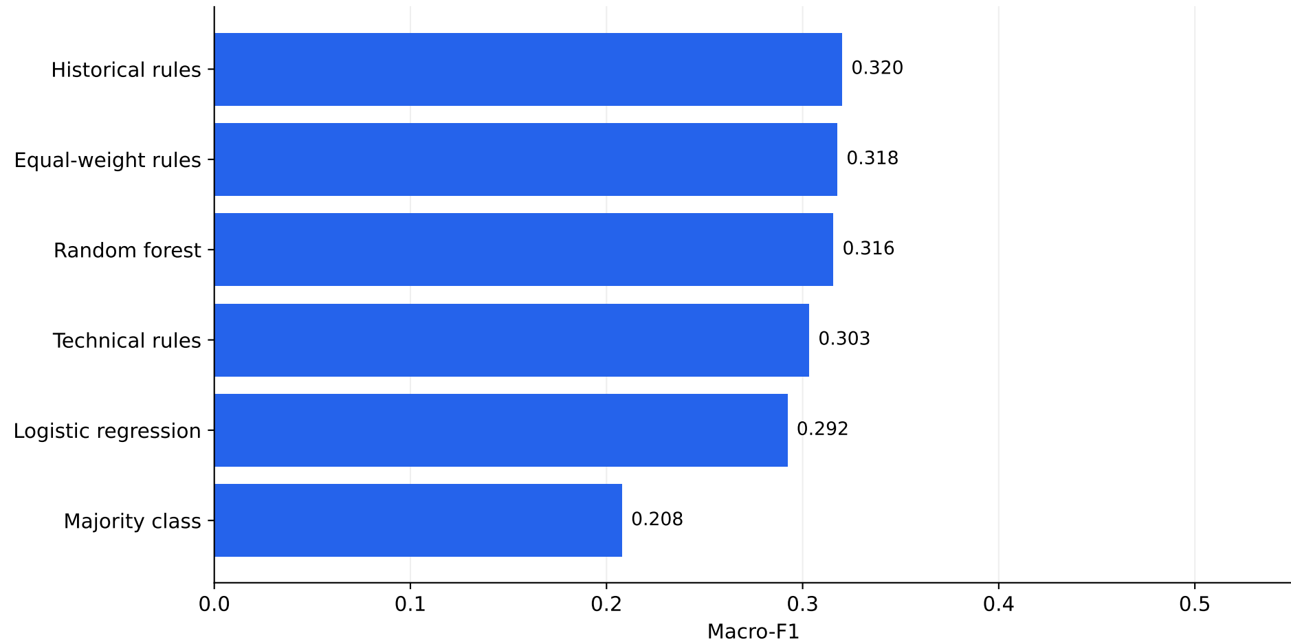
Four-market price models — 2025 holdout (490 observations)
