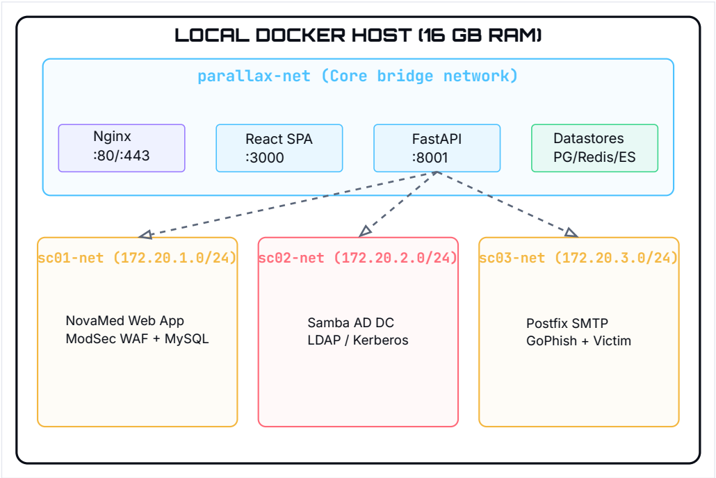
Figure 3 · 12 — Docker host deployment and isolated container subnet topology
