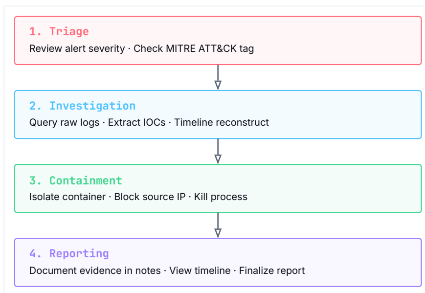
Figure 5 · 3 — Blue-Team incident response workflow: from SIEM alert to reporting
