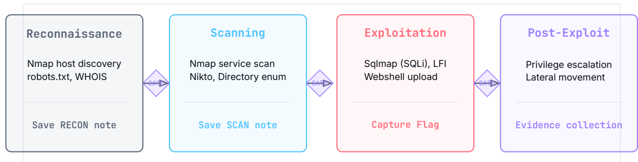
Figure 5 · 2 — Red-Team offensive methodology flow and notes check-gates
