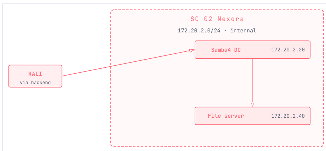
Figure 5 · 7 — SC-02 Nexora topology (Active Directory)
