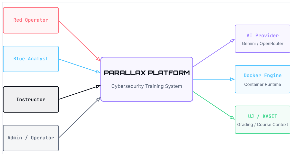
Figure 3 · 2 — PARALLAX use-case model: four actors over one shared system
