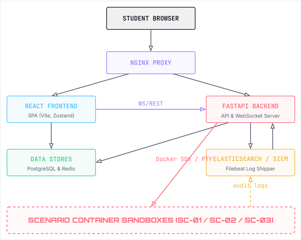
Figure 3 · 6 — PARALLAX C4 container diagram: system containers, protocols, and data routes
