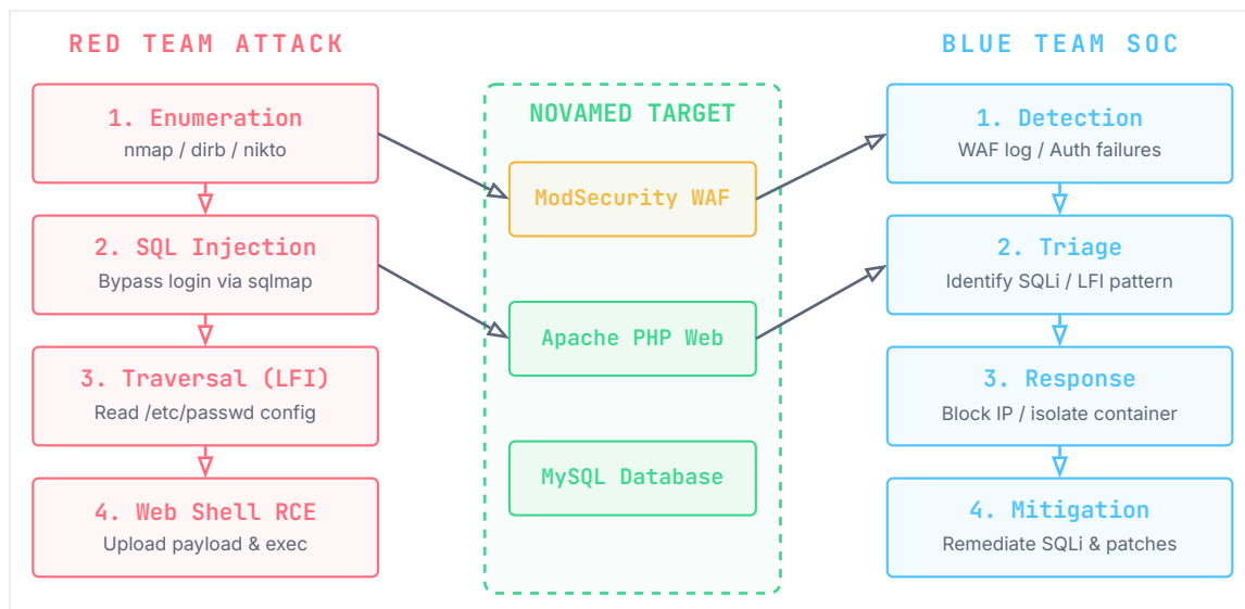
Figure 5 · 6 — SC-01 NovaMed attack-defense telemetry correlation flow
