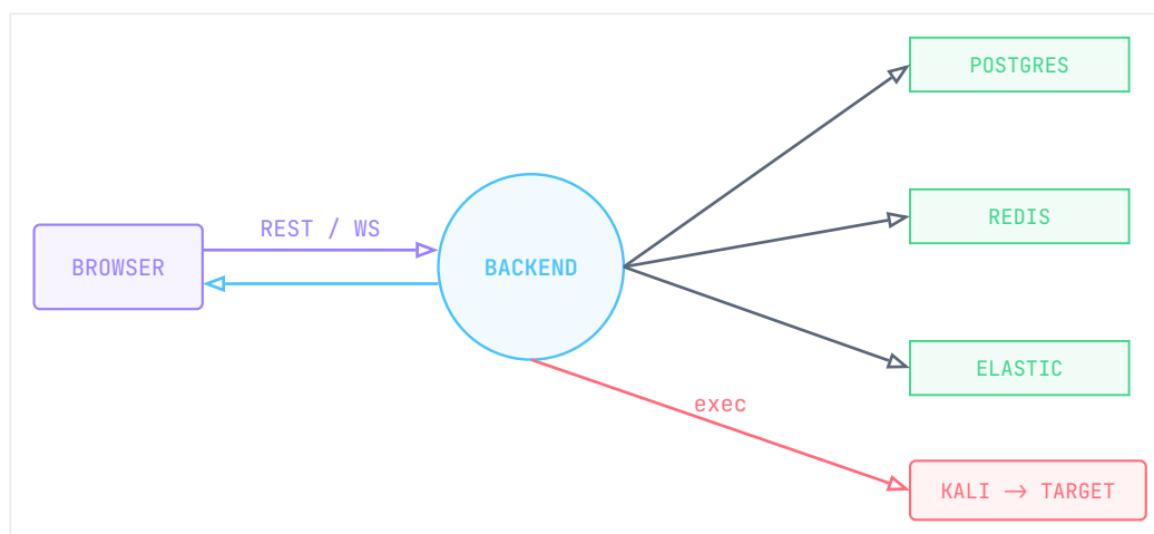
Figure 3 · 8 — Level-0 data flow across browser, backend, stores, and sandbox
