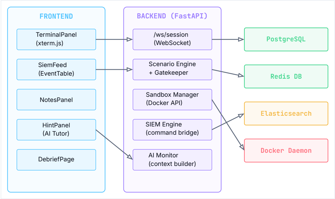
Figure 3 · 7 — Detailed component interaction model across frontend, backend, and data layers
