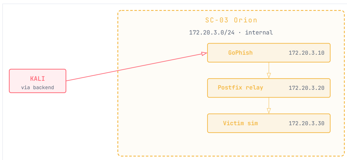
Figure 5 · 8 — SC-03 Orion topology (phishing campaign)
