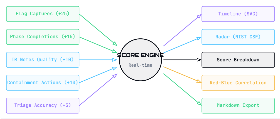
Figure 5 · 9 — Scoring engine data ingestion and debrief visualization pipeline
