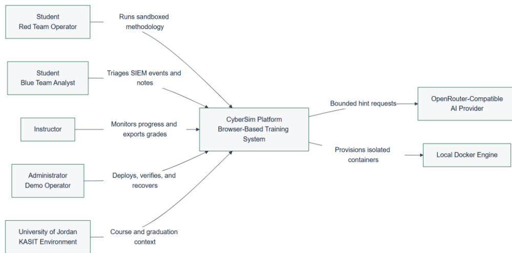
Figure 4.1: CyberSim System Context (C4 Level 1)
