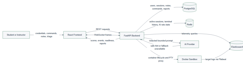
Figure 4.3: CyberSim Data Flow Diagram (Level 0)
