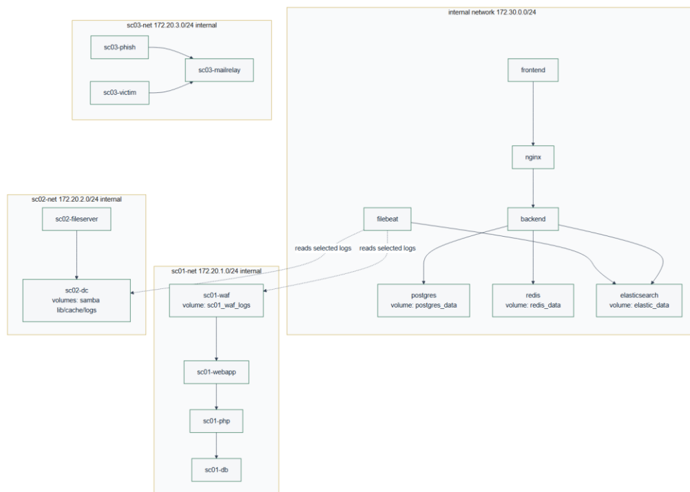
Figure 4.5: Docker Network and Service Topology
