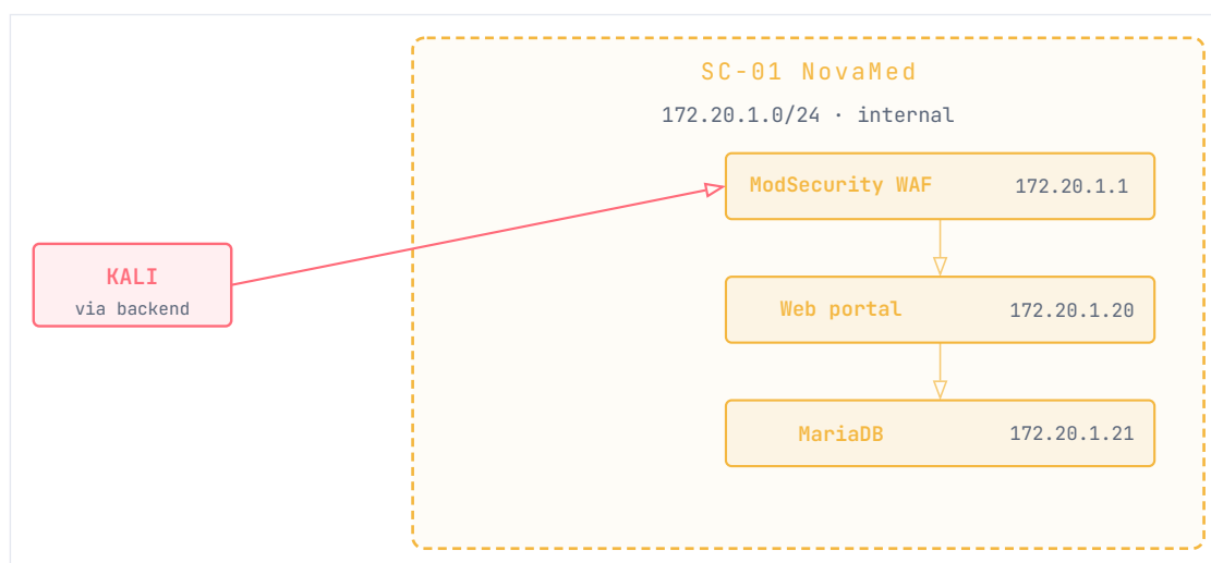
Figure 5 · 5 — SC-01 NovaMed topology (web application + WAF)
