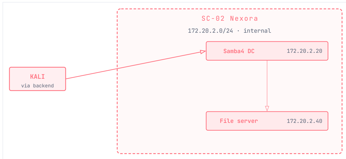
Figure 5 · 5 — SC-02 Nexora topology (Active Directory)
