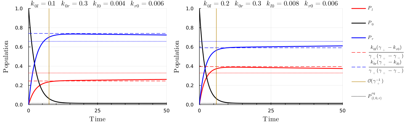
FIG. S6. Toy example of the population dynamics for the triple well rate equation P_l \xrightleftharpoons[k_{l0}]{k_{0l}} P_0 \xrightleftharpoons[k_{r0}]{k_{0r}} P_r . The dotted lines are the equilibrium distributions while the dashed lines are the kinetic yield.
