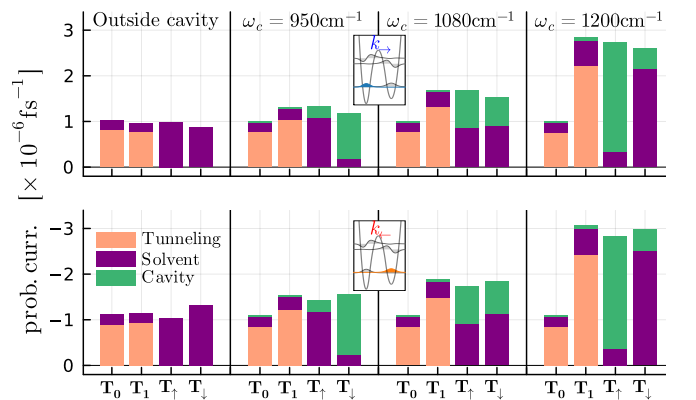
FIG. 6. The associated probability currents for both the k_{\rightarrow} (top) and k_{\leftarrow} (bottom) reaction dynamics of the least asymmetric system in figure 5. Probability currents for the other systems can be found in Supplementary Fig. S8.
