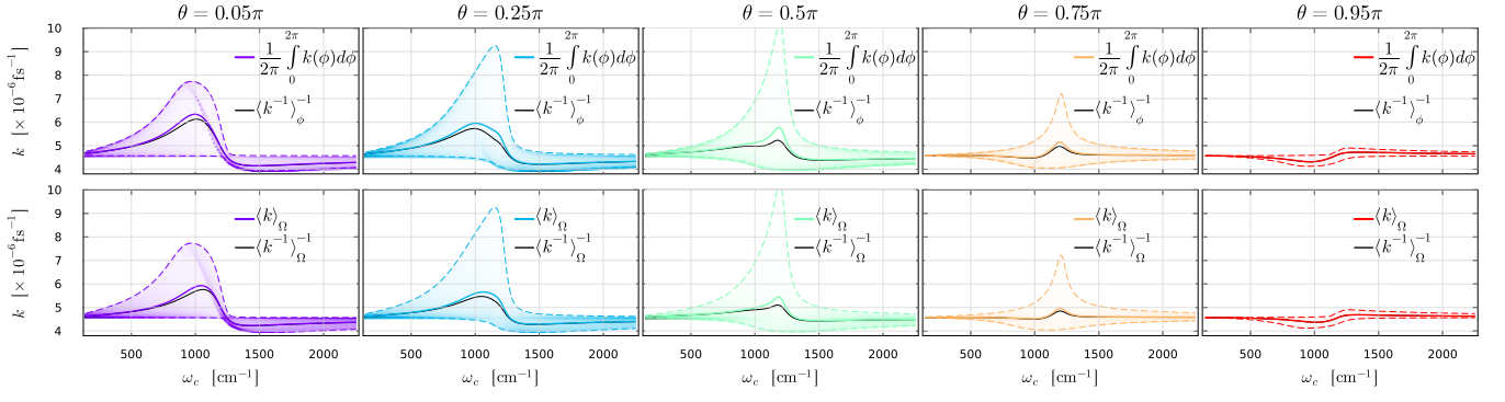
FIG. S3. Distribution of reaction rates p(k) for an ensemble of molecules with random orientations, visualized by shaded rate profiles. The rate is calculated from Eq. 28 and the distribution of the molecule orientations is either uniform in the plane containing the cavity polarization (top panel) or isotropic in 3-dimensions (lower panel). The dashed lines represent the minimum and maximum rates and the full colored line is the mean \langle k \rangle while the black line is the asymptotic reaction rate \langle k^{-1} \rangle^{-1} = \left( \int_0^\infty p(k) k^{-1} dk \right)^{-1} . Fitting a single exponential to the decay curve of such an ensemble, would yield a reaction rate in between these two limits.
