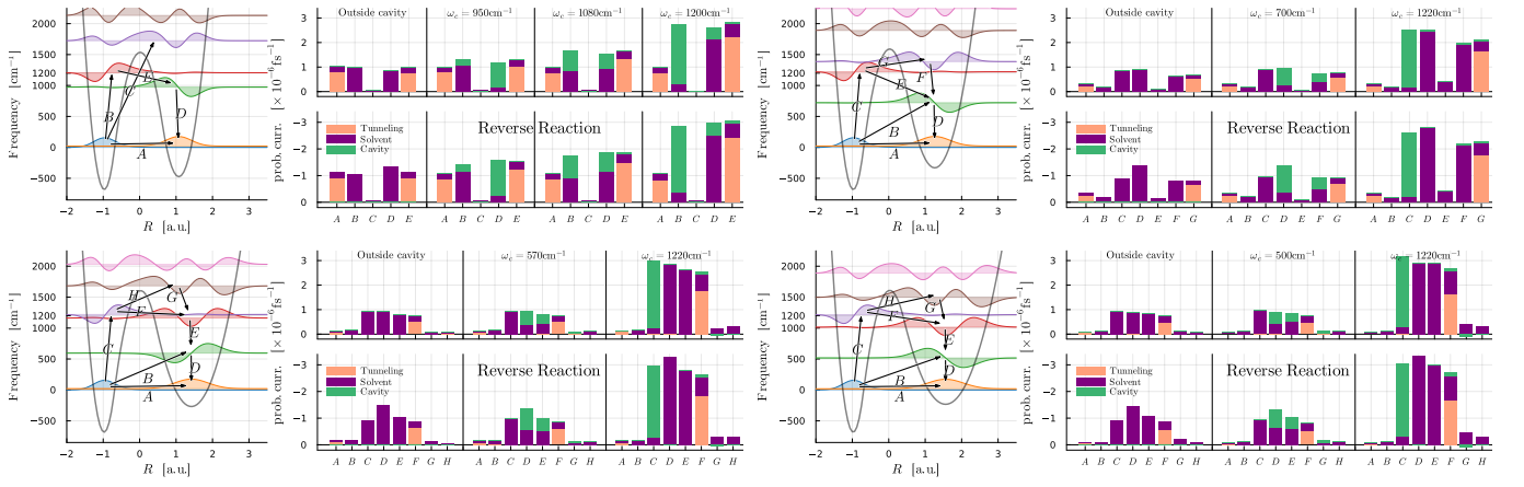
FIG. S8. Probability currents for the asymmetric double wells. A negative rate means that the current goes in the opposite direction of the arrow. All currents with magnitude larger than 0.05 \times 10^{-6} \text{fs}^{-1} are shown.
