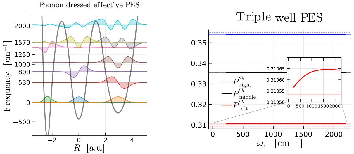
FIG. S4. (left) Visualization of the phonon-dressed vibrational states of the reaction coordinate according to the diagonalization of \tau_{MF} described in Sec. S8. (right) Comparison of the population in the left (red), middle (black) and right (blue) wells at equilibrium. The dotted lines are the predictions from the Gibbs state \tau \propto e^{-\beta H_R} . The solid lines include the correction from the structured environment via Eq. S83, for which the horizontal line is for outside the cavity while the thicker line includes the cavity contribution.
