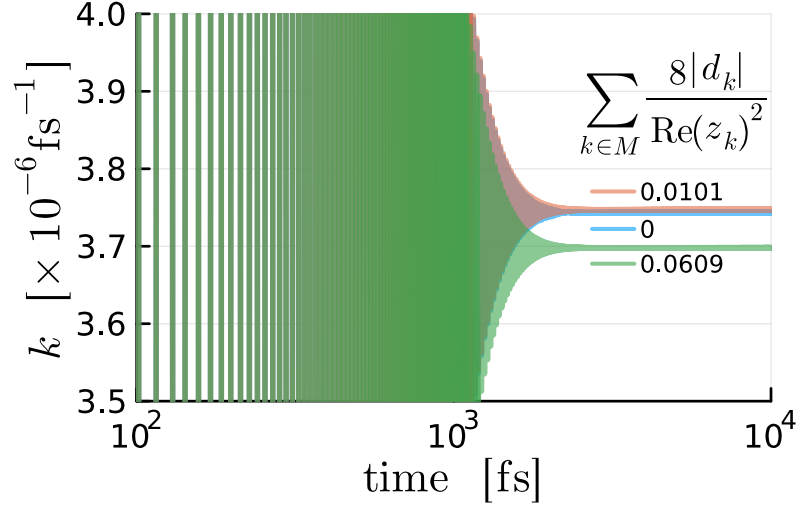
FIG. S2. Comparison of k(t) = \frac{\dot{P}_r(t)}{1-2P_r(t)} (Eq. S53) for different levels of Markovian compression of the phonon bath. See Table I for an overview of the results. The observed oscillations correspond to the inherent time scale of the phonon bath \gamma_R^{-1} \approx \beta \approx 25\text{fs} and originates from the quenched dynamics since the system is initialized in a product state with the phonon bath. The simulations were carried out using tensor networks, and for this environment, the number of physical indices needed to represent the environment could be reduced from 2 \times 19 = 38 to 2 \times 2 = 4 without having any effect on the observed reaction rate. This should be compared to reducing the number of indices by performing a less accurate decomposition of the bath correlation function in terms of only two exponentials, which would result in a larger deviation in the observed rate.
