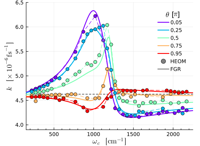
FIG. 9. Numerically exact reaction rates compared to predictions calculated via Eq. 28. The Lorentzian has parameters \omega_0 = 1205\text{cm}^{-1} and \Gamma = 30\text{cm}^{-1} and the approximate scaling factor was rescaled \frac{1}{2} \rightarrow 0.38 to best match the results from HEOM. The horizontal dashed line correspond to the reaction rate outside the cavity.
