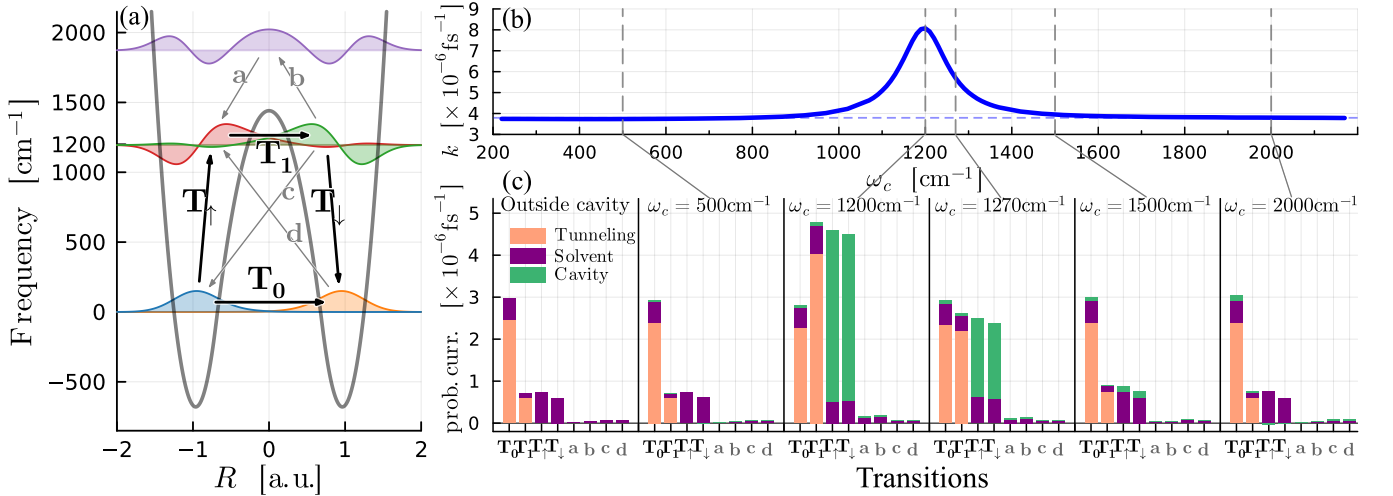
FIG. 4. (a) The wavefunction of the localized states of the reaction coordinate visualized alongside the potential with the y-axis providing the energy difference to the ground state. The transitions between these states are labeled and visualized by arrows. (b) Reaction rate profile when varying the cavity frequency compared to the out-of-cavity reaction rate (horizontal dashed line). Due to the symmetry of the PES, the forward and backward reaction rates are equal k := k_{\rightarrow} = k_{\leftarrow} . (c) The probability current at t = 6 \text{ps} for the labeled transitions as a function of the cavity frequency. The probability currents are decomposed in terms of contributions from the system Hamiltonian (tunneling) and from coupling to bath degrees of freedom (solvent and cavity).
