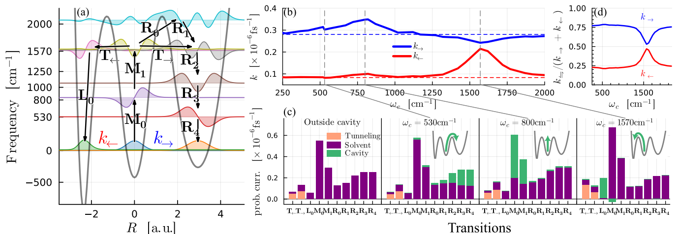
FIG. 7. (a) Visualization of the triple well PES and the vibrational states. The middle well is the reactant region and k_{\leftarrow} and k_{\rightarrow} denote the reaction rate to the left and right product wells, respectively. The black arrows label the state-to-state transitions. (b) Shows the reaction rates at different cavity frequencies. The horizontal dashed lines denote the rates outside the cavity. (c) Probability currents for the associated transitions, both outside and inside the cavity. (d) The inferred kinetic yield of the left product in red and the right product in blue for different cavity frequencies. This does not constitute the yield at equilibrium, which remains largely unaffected by the presence of the cavity.
