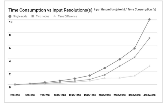
Figure 2 : Comparison of IWP on Single device vs Two Devices
