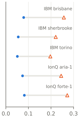
(b) deficit error, trained circuits
