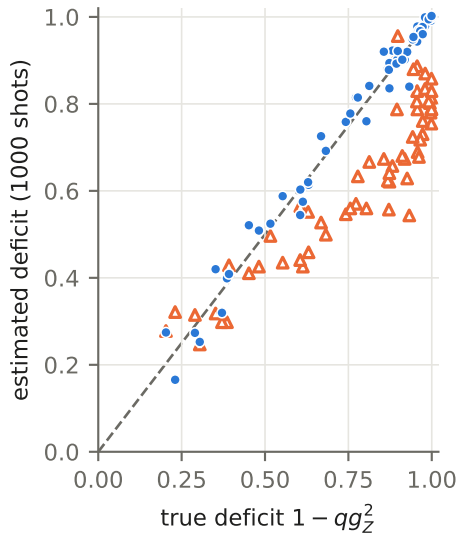
(a) equal T1, 6 qubits, weight 2, depth 24
