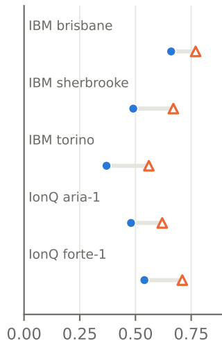
(c) false deficit, product states (echo)
