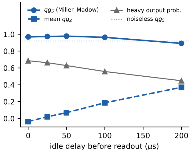
(b) fake_brisbane calibration noise, 4000 shots
