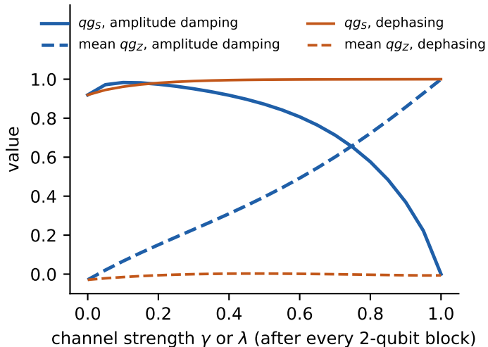
(a) idealized channels, exact
