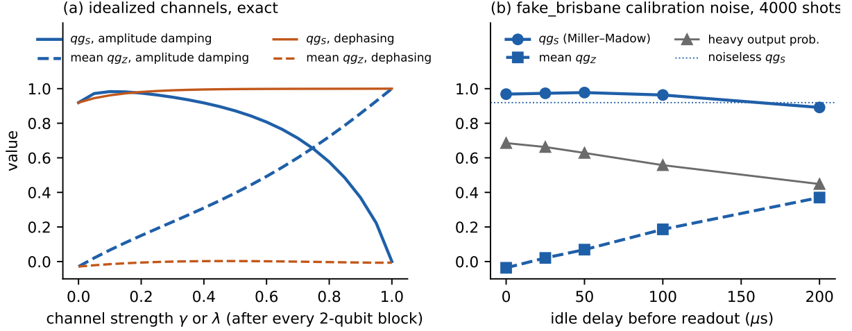
Figure 1: (a) 4-qubit Quantum Volume circuit, exact density-matrix simulation with amplitude damping or dephasing after every two-qubit block. qg_S is non-monotonic under amplitude damping, while the mean qg_Z separates the regimes. (b) The same circuit under fake_brisbane calibration noise with an idle delay before readout. Heavy output probability and mean qg_Z are monotonic; qg_S falls below its noiseless value (dotted).
