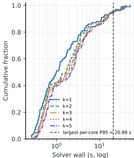
Solver-wall ECDF
