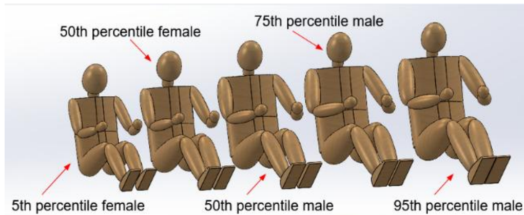
Figure 1: Wilson models used to determine driver clearance. All are same proportion and scaled to match the height of a potential driver.
