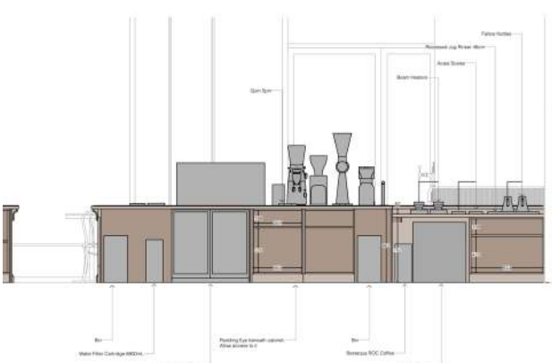
02/ Elevation B2
