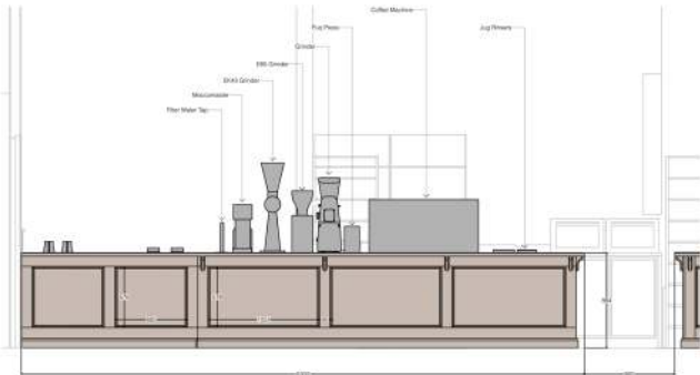
01/ Elevation A
