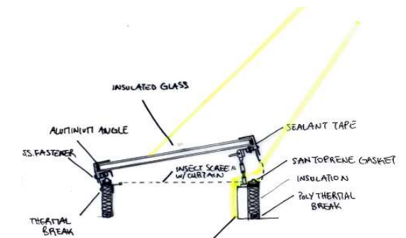
NW view Manual opening of skylight in artists' studio
