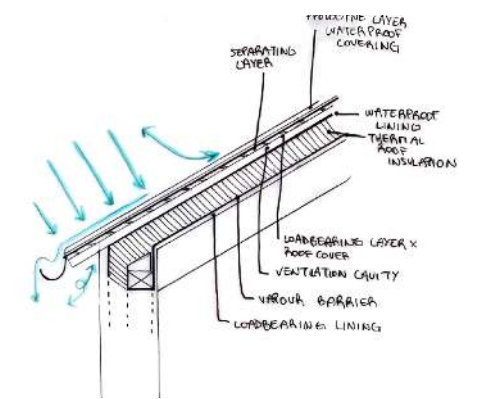
NE view Roof detail throughout pitched roofs in the building
