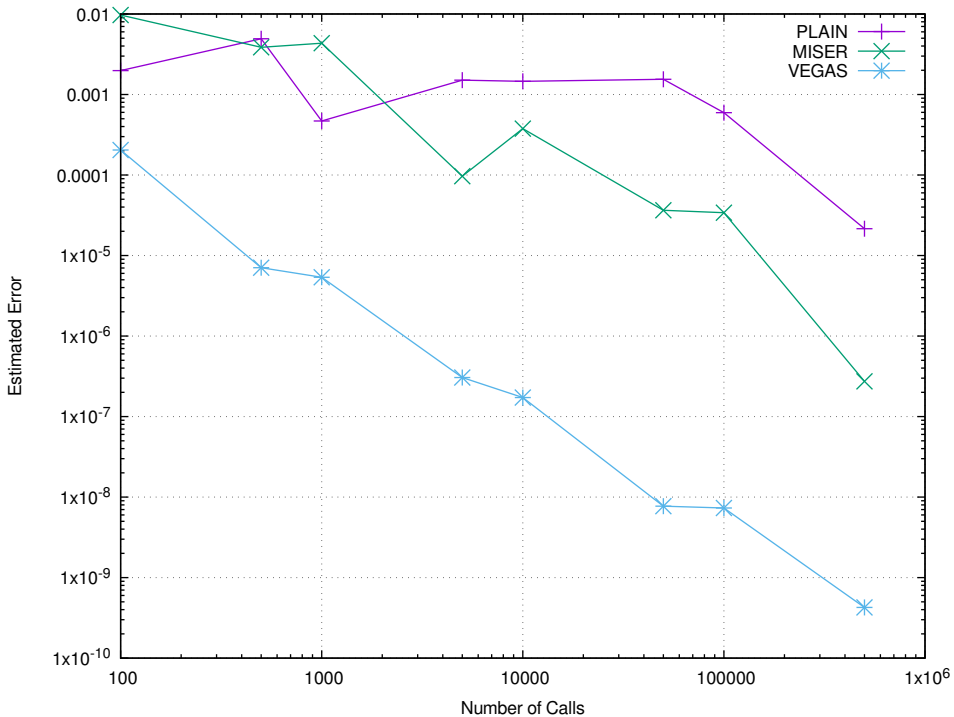
GSL Methods Error: f_2(x) = \sqrt{1-x^2}
