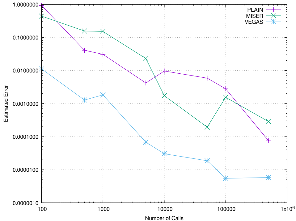
GSL Methods Error: f_3(x) = 1/\sqrt{x}
