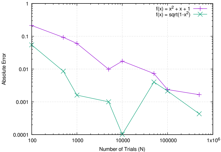
Hit-and-Miss Integration Error vs. Number of Trials
